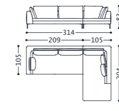
01CL2C2 (1CL2D2MSX - 1CL2CHLDX) 02CL2C2 (2CL2D2MSX - 2CL2CHLDX)
